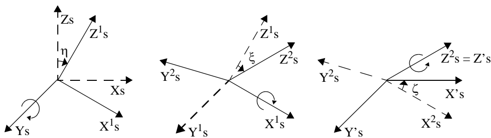
Figure 3: Euler Angles
