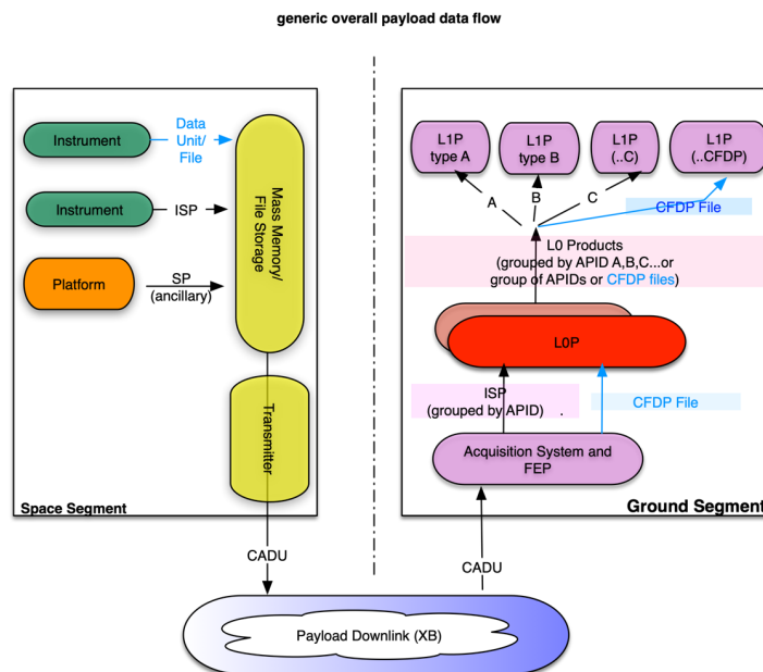
Fig. 3. Ideal dataflow in ESA EO Ground System
