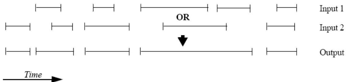
Figure 11: xv_timesegments_compute_or function
