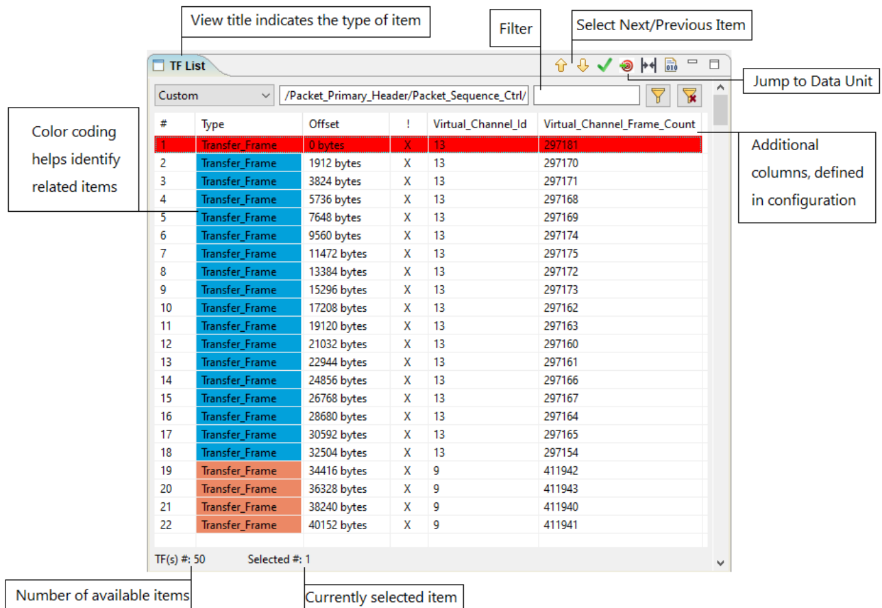
Figure 11: Details of the Data Unit List View
