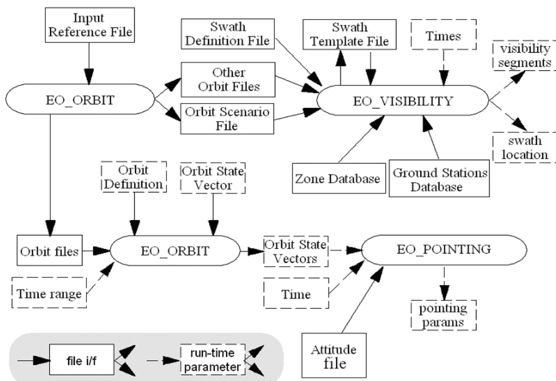
Figure 3: EO_ORBIT, POINTING and VISIBILITY data flow
