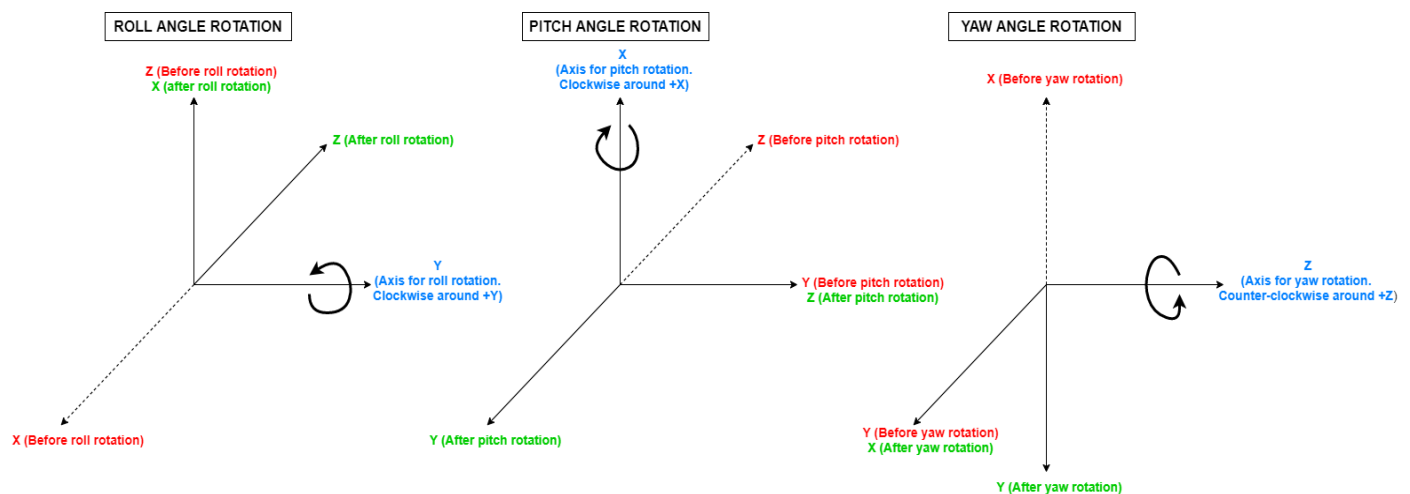
Figure 4: Euler Angles
