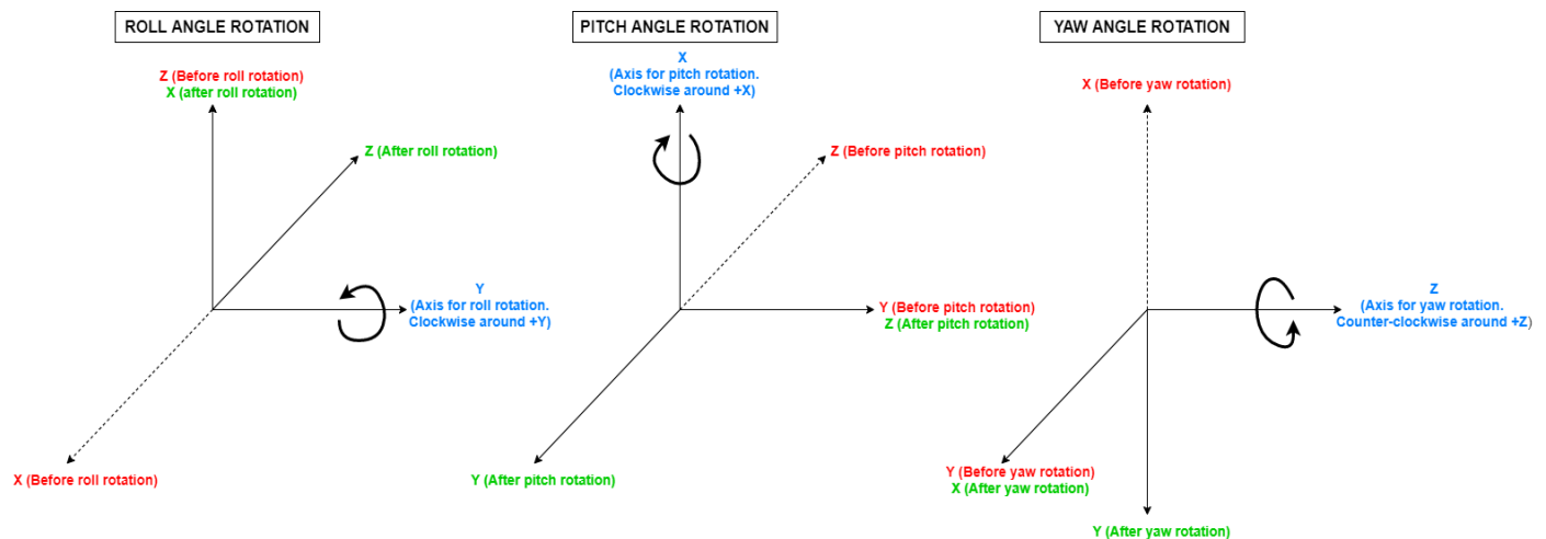
Figure 4: Euler Angles
