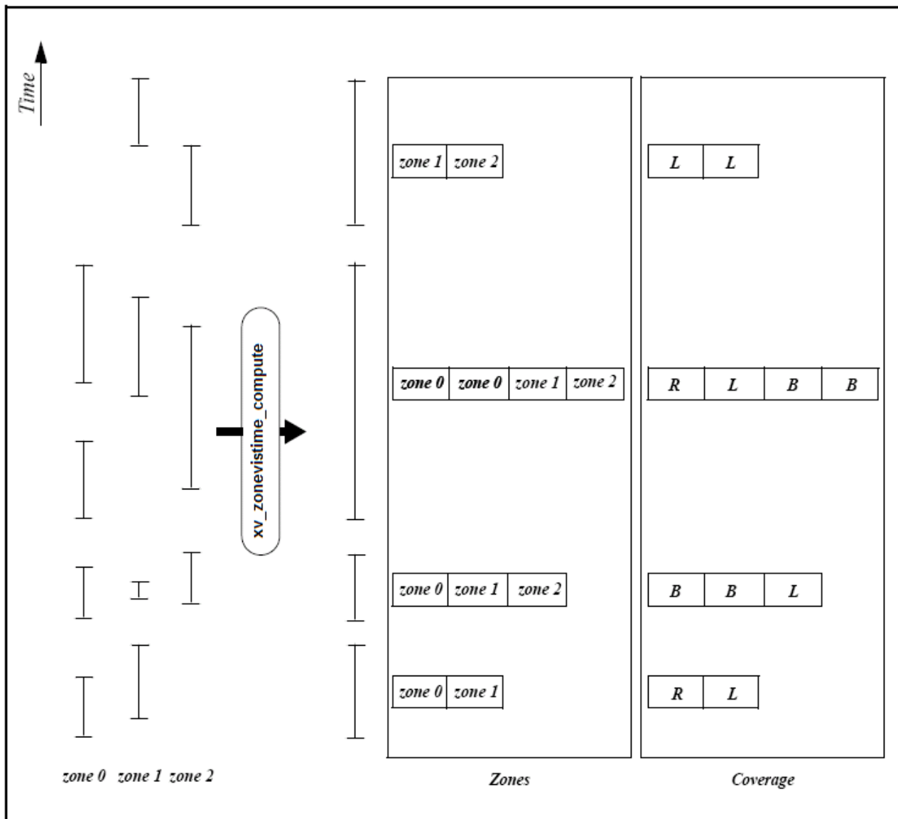
Figure 6: xv_zonevstime_compute function (more than one zone)
