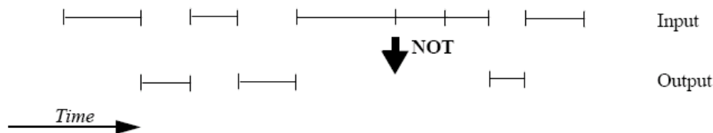
Figure 10: xv_timesegments_compute_not function
