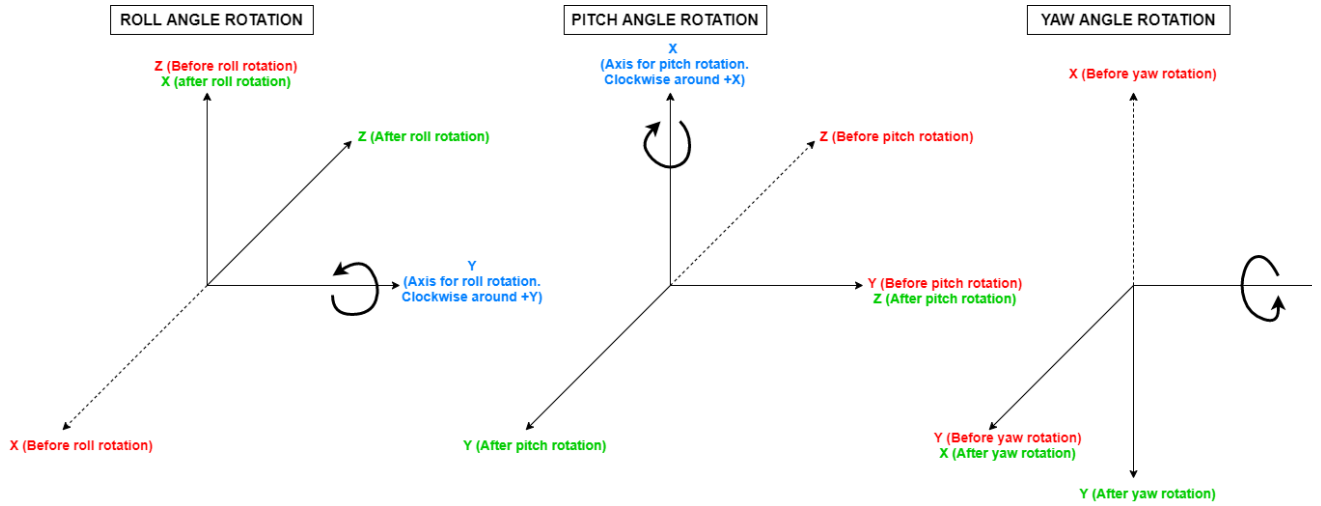
Figure 16: Euler Angles
