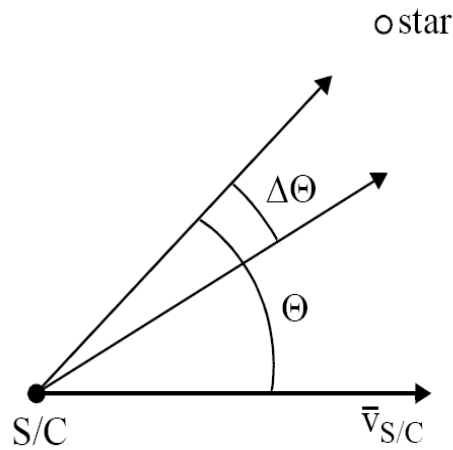
Figure 17: Satellite aberration
