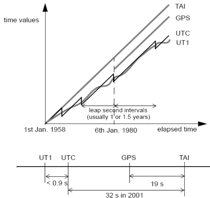
Figure 1: Relationships between UT1, UTC and TAI
