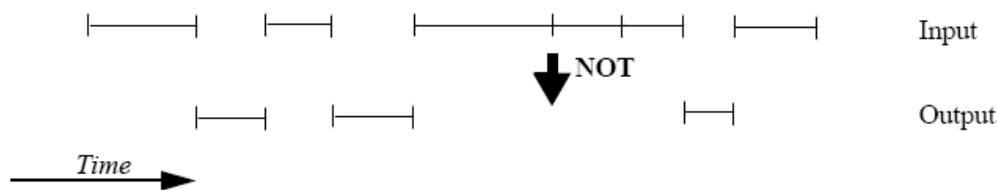
Figure 23: xv_timesegments_compute_not function
