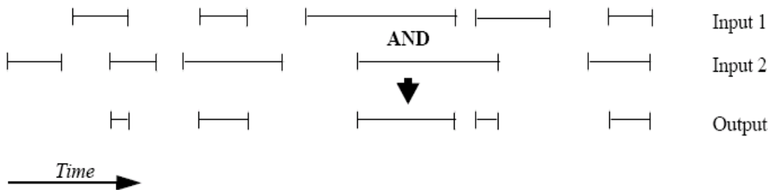
Figure 26: xv_time_segments_and_function
