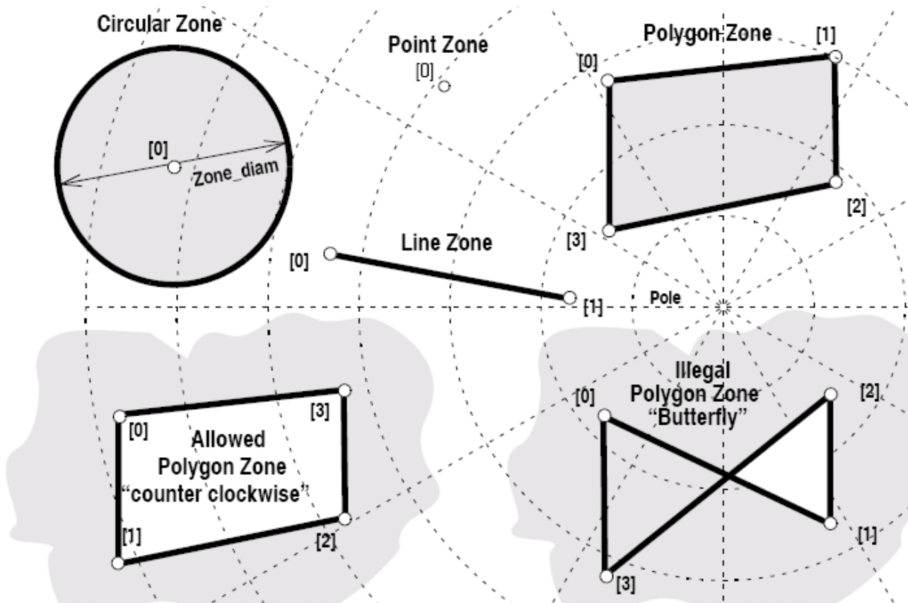
Figure 6: Zone examples
