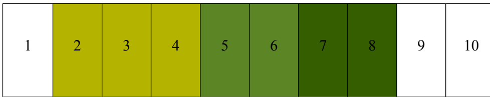
Fig. 7 Cumulative Coverage
