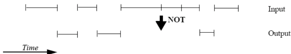
Figure 22: xv_time_segment_not_function
