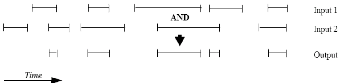
Figure 12: xv_timesegments_compute_and_function
