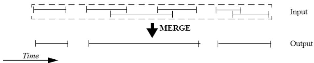
Figure 13: xv_timesegments_compute_merge function
