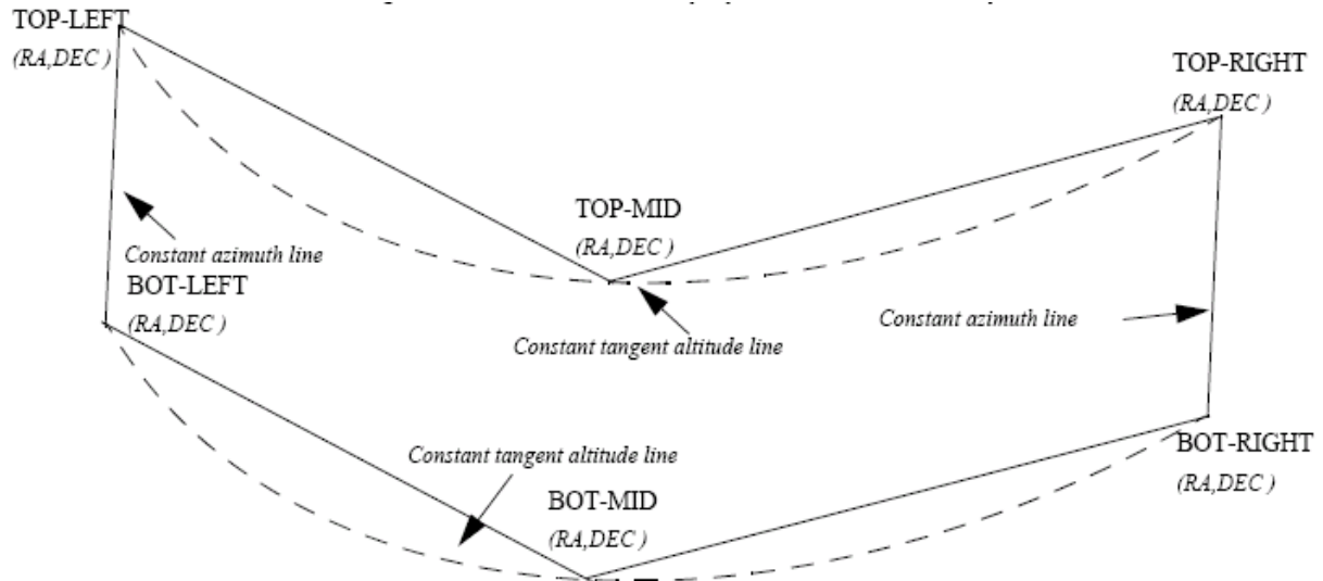
Figure 9: Instantaneous FOV projected on the celestial sphere
