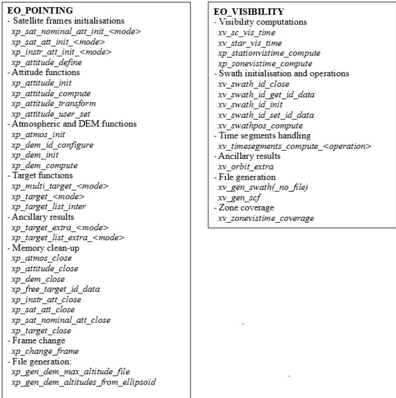
Figure 1: Earth Observation CFI Software libraries
