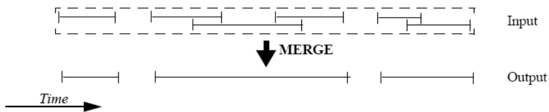
Figure 13: xv_timesegments_compute_merge function
