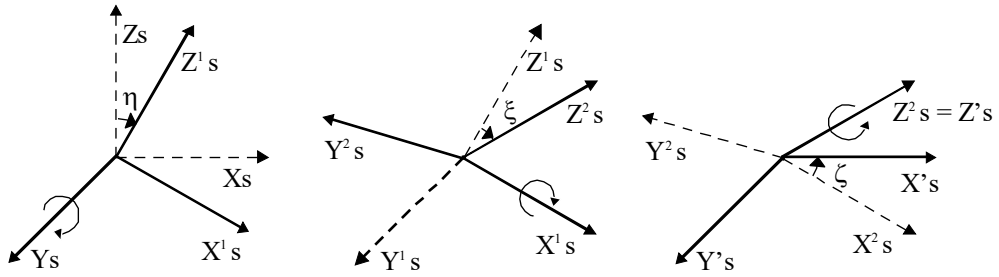
Figure 16: Euler Angles
