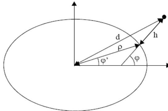
Figure 13: Geodetic position
