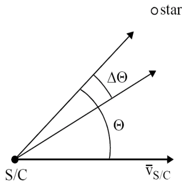
Figure 17: Satellite aberration
