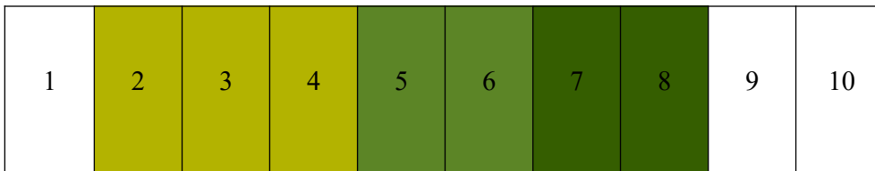
Fig. 7 Cumulative Coverage
