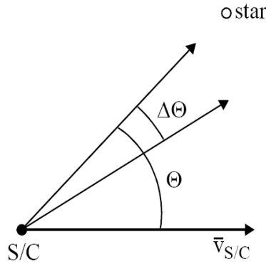
Figure 17: Satellite aberration
