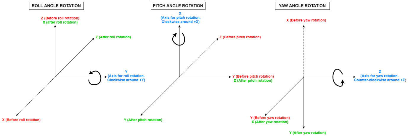
Figure 16: Euler Angles
