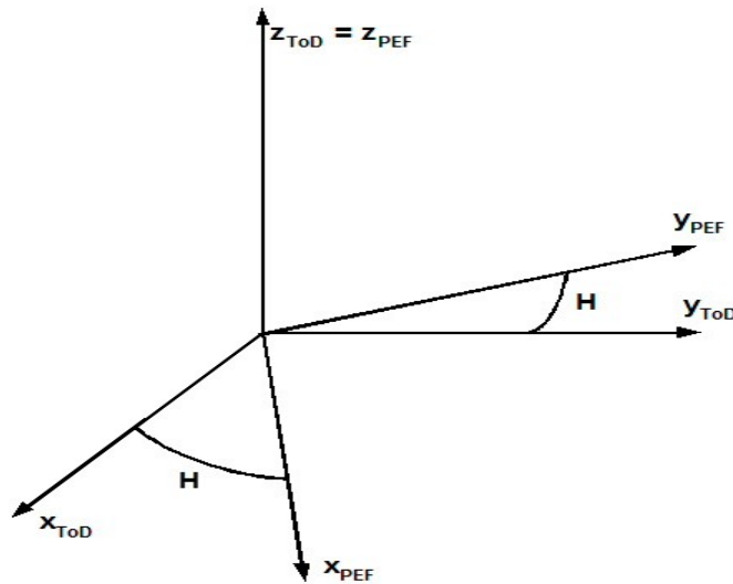
Figure 8: Transformation between ToD and PEF reference frames
