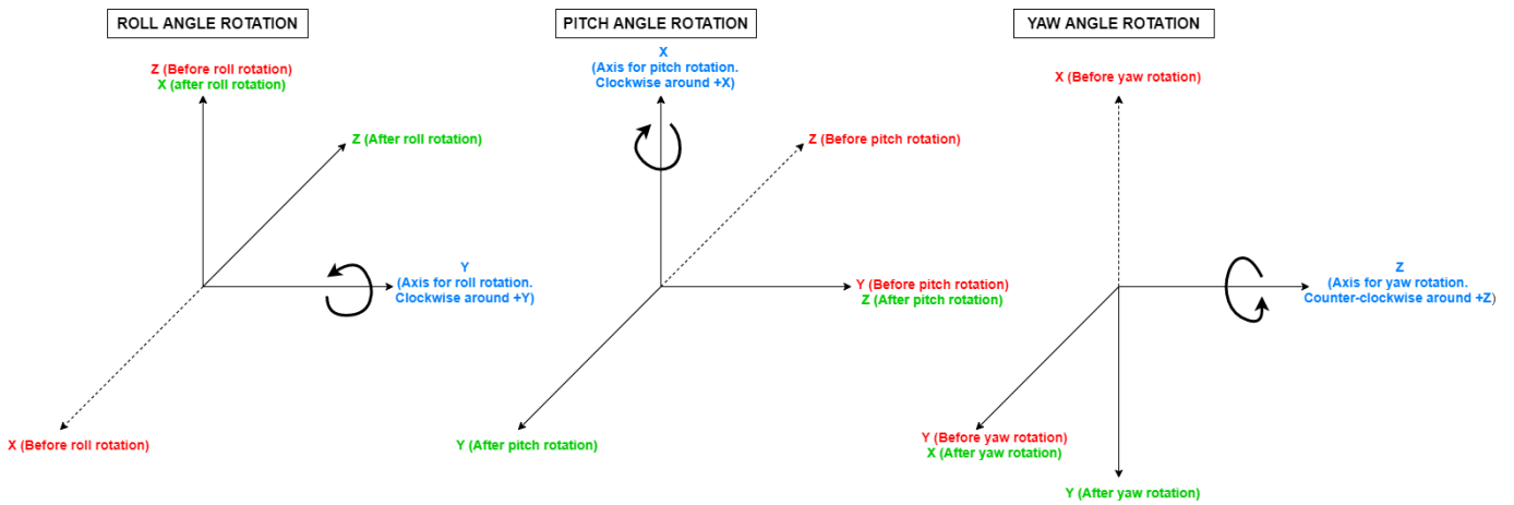
Figure 16: Euler Angles
