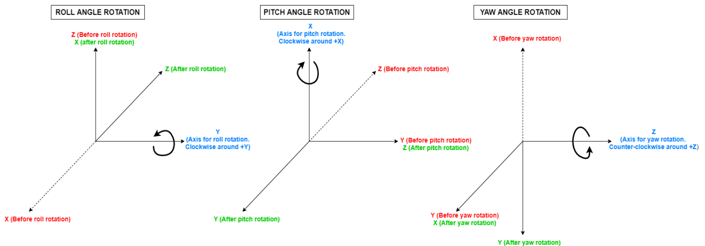
Figure 4: Euler Angles
