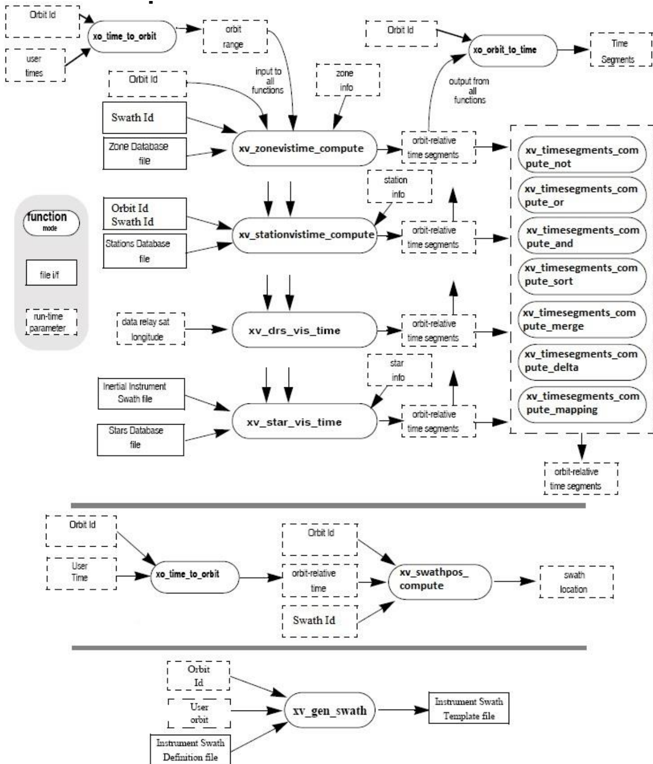
Figure 1: EO_VISIBILITY Data Flow
