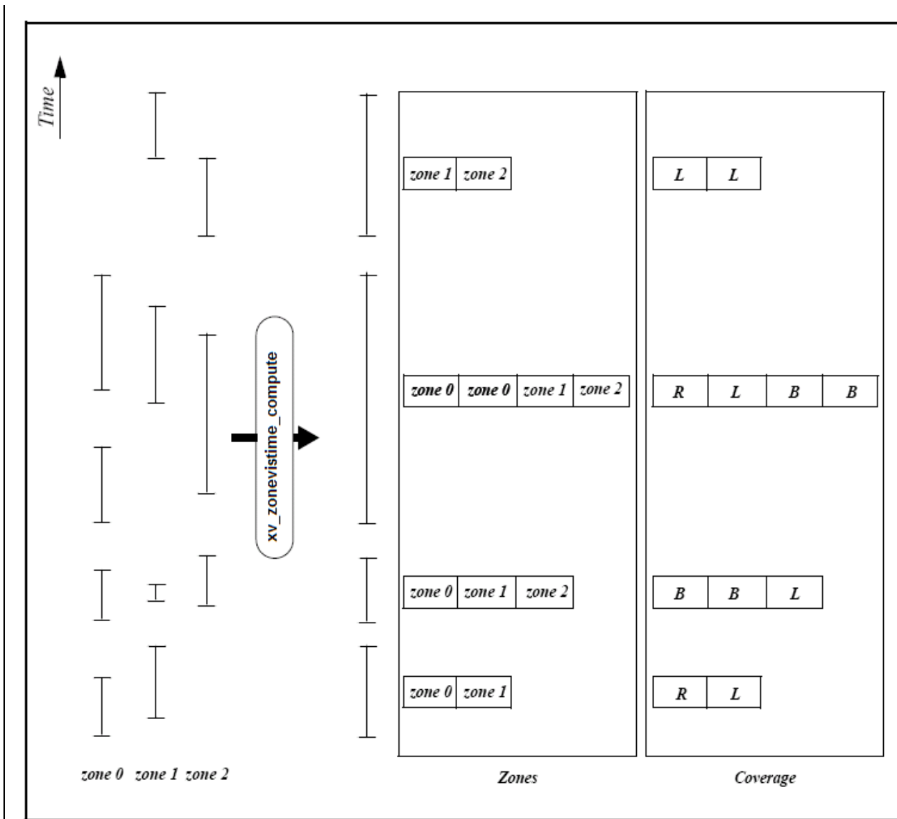
Figure 6: xv_zonevistime_compute function (more than one zone)
