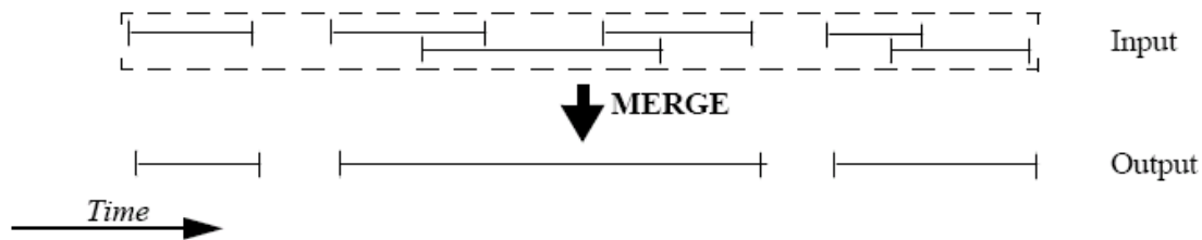
Figure 16: xv_time_segments_merge function
