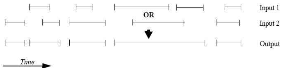
Figure 25: xv_timesegments_compute_or function
