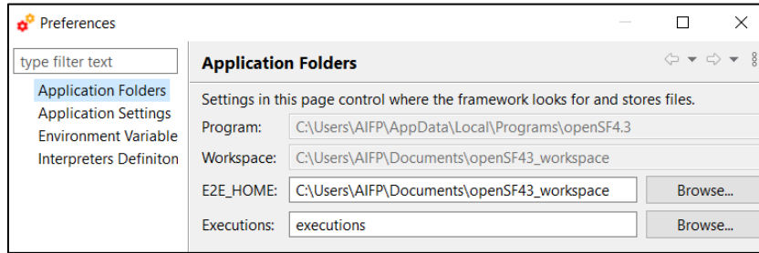
Figure 4-154: Application folders
