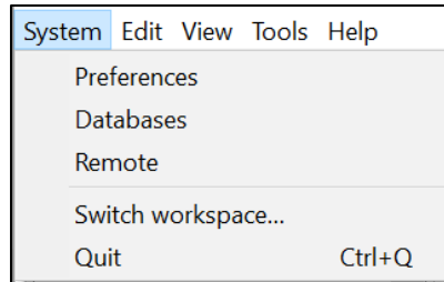
Figure 4-150: System Menu
