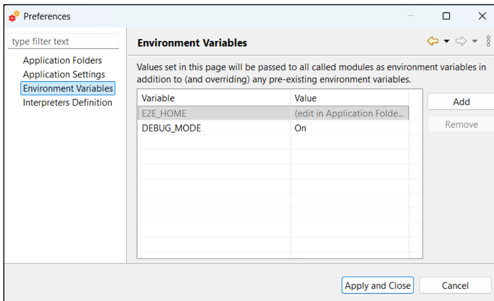
Figure 4-151: Environment variables
