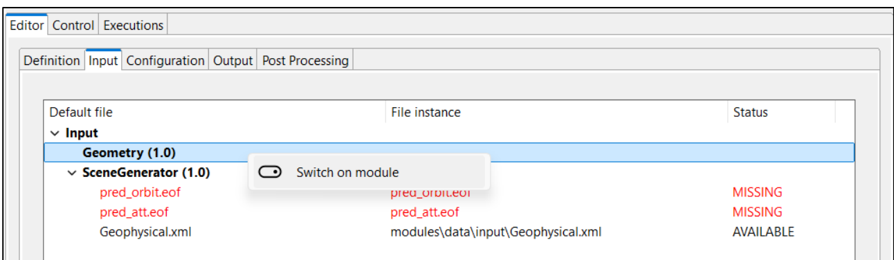
Figure 4-88: Switch-on module
