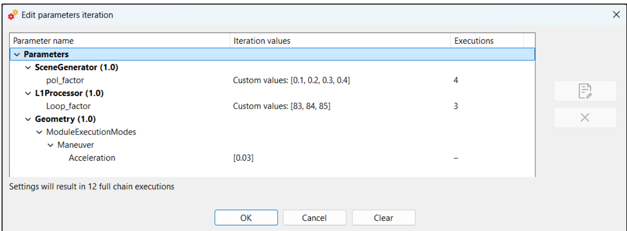
Figure 4-94: Iterating parameters
