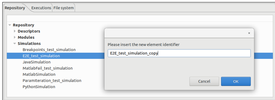
Figure 4-43: Simulation copy
