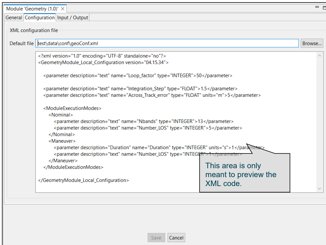
Figure 4-37: Module configuration
