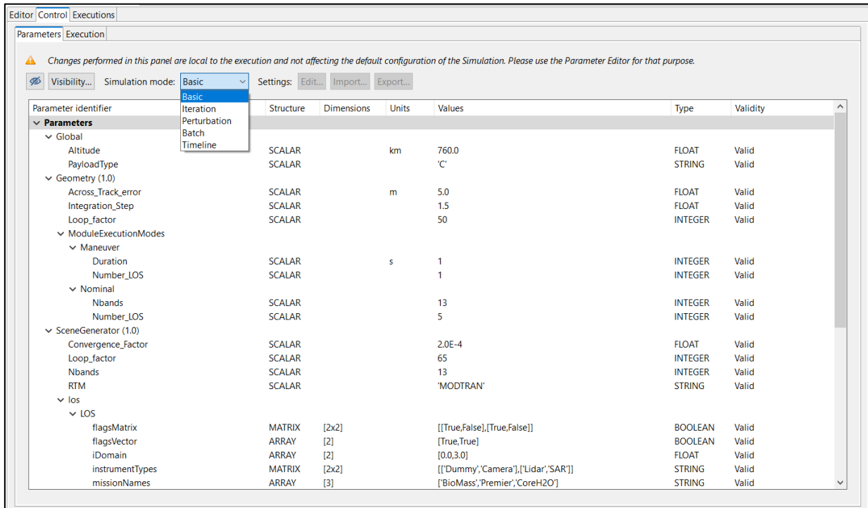
Figure 4-93: Parameters view
