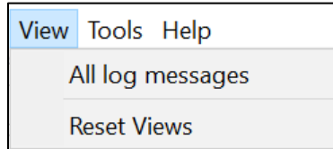
Figure 4-135: Logs menu
