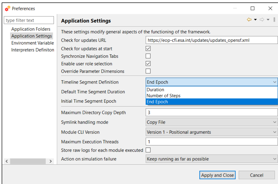
Figure 4-116: Timeline preferences
