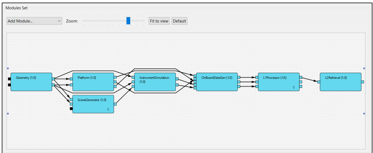
Figure 4-46 Simulation diagram
