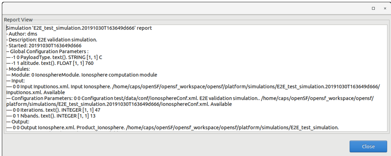
Figure 4-71: Execution report
