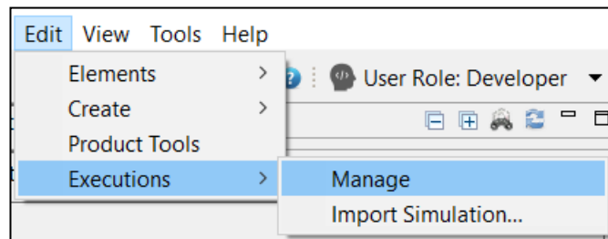
Figure 4-64: Results menu
