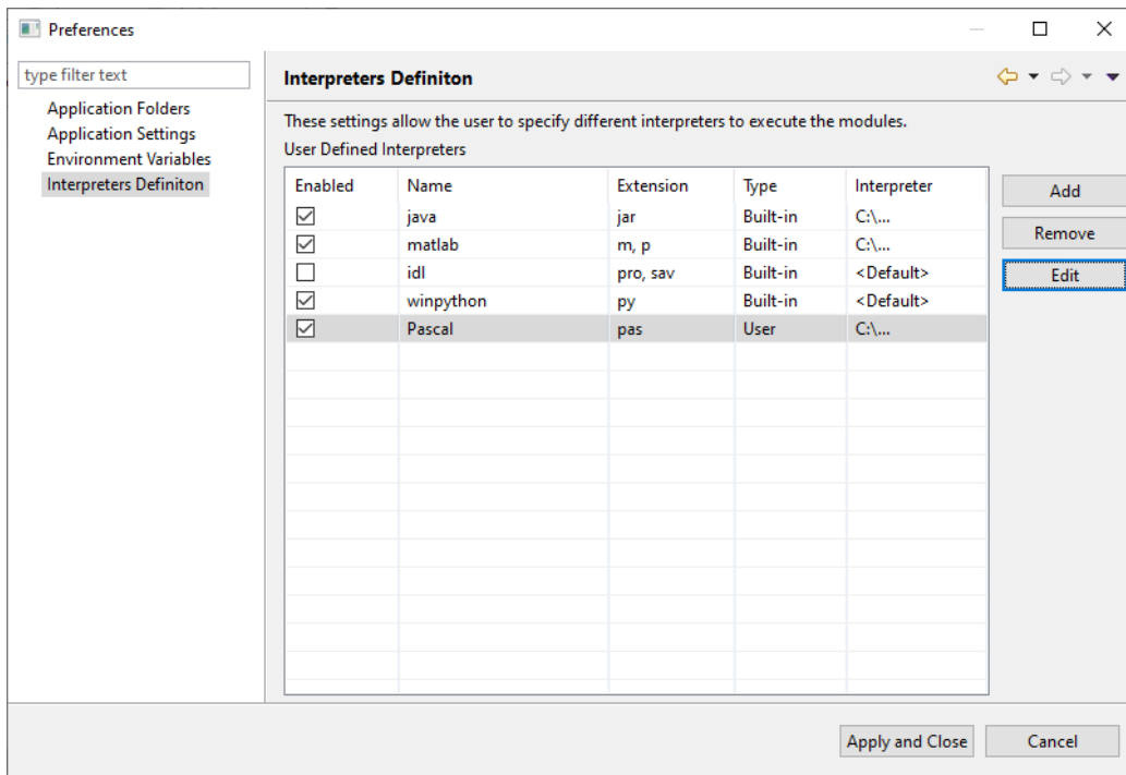
Figure 4-156 Interpreters definition
