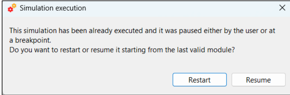
Figure 4-70: Result. Re-run
