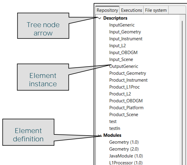
Figure 4-6: Repository view
