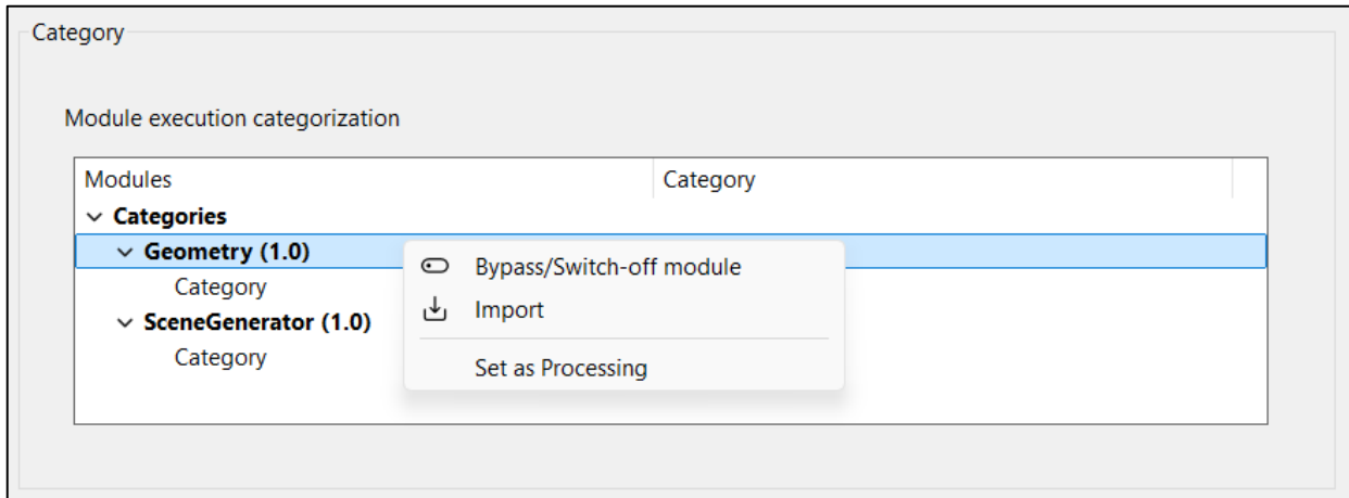
Figure 4-86: Bypass/Switch-off module
