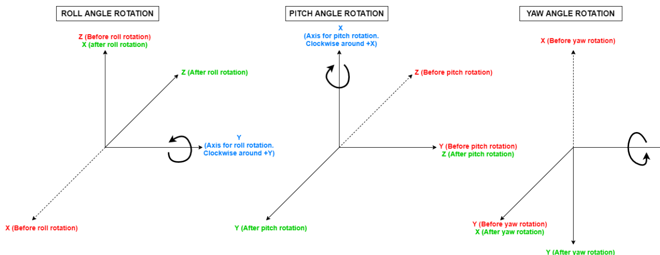
Figure 16: Euler Angles
