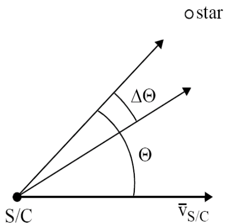
Figure 17: Satellite aberration
