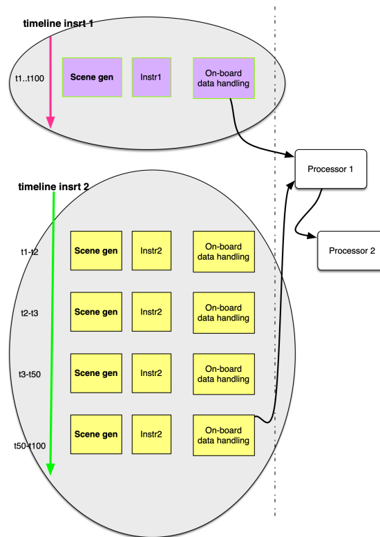
Figure 3-3 - Multi-Instrument E2E simulation with different timelines for each instrument
