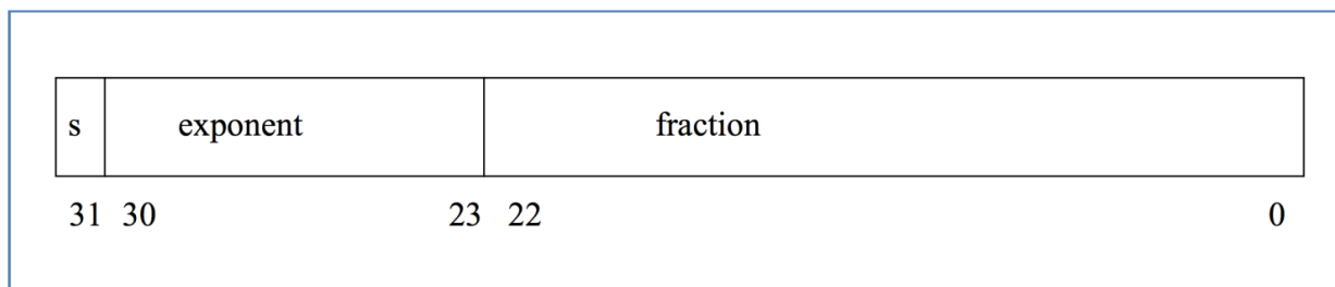
Figure 6.3-2 Single-precision Floating Point Storage Format
