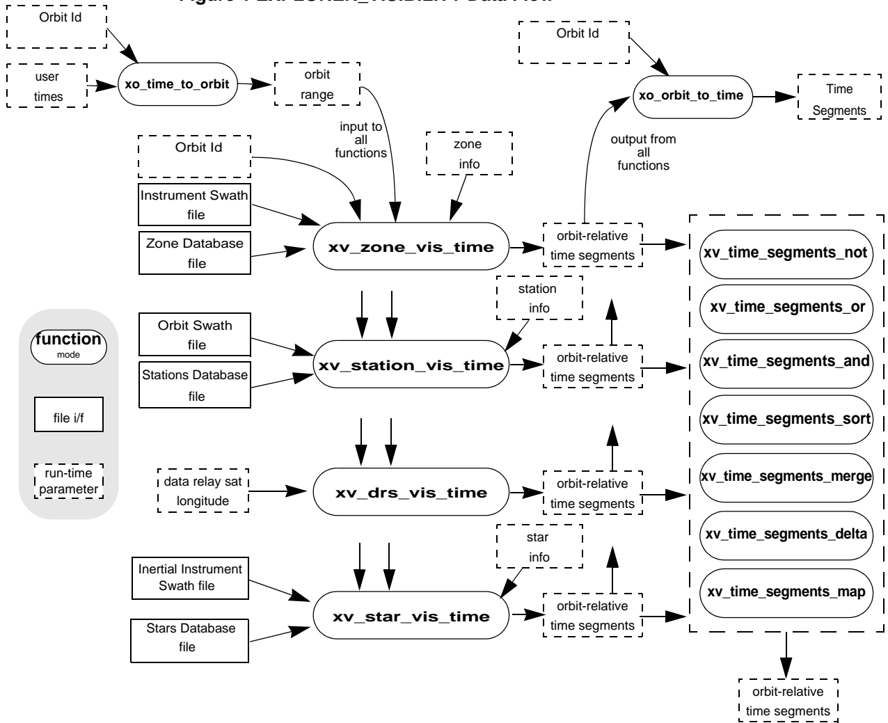
Figure 1 EXPLORER_VISIBILITY Data Flow
