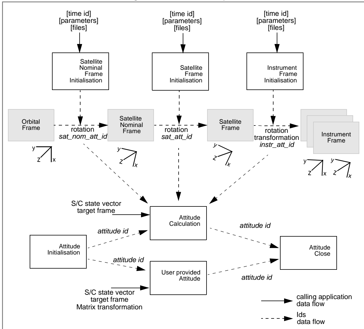
Figure 9: Attitude data flow
