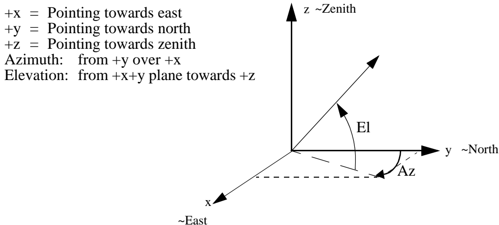
Figure 14: Topocentric direction
