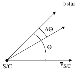
Figure 16: Satellite aberration
