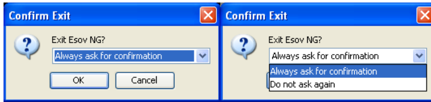
Figure 4.3: Exit Dialog
