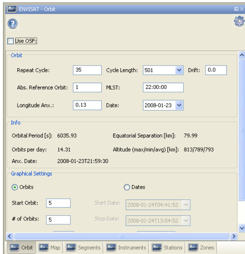
Figure 4.9: Toolwindows arranged as dockable components (example)
