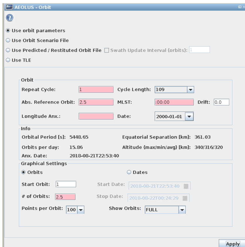
Figure 5.4: Invalid orbit definitions
