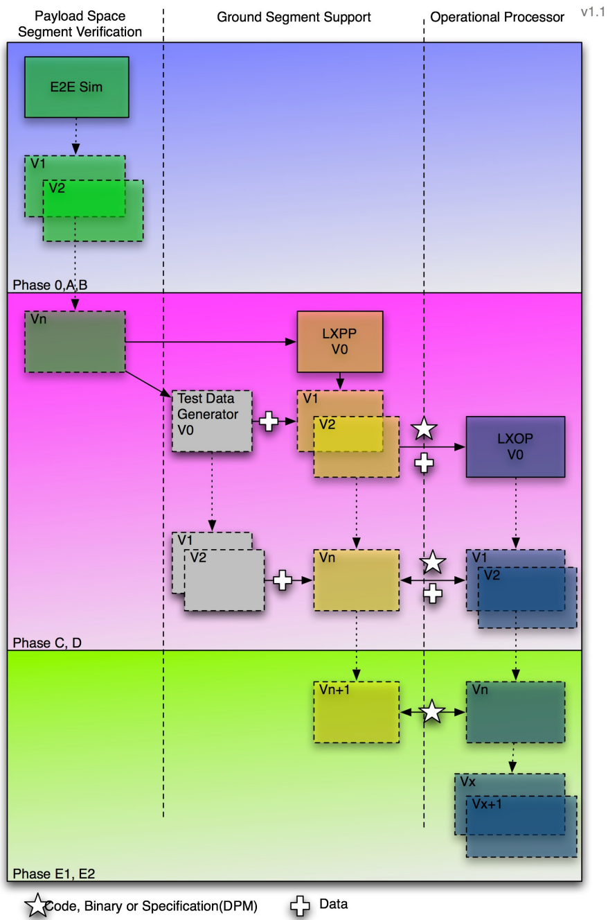
Fig. 3-2: Typical evolution of the E2E Performance Simulator and L1PP
