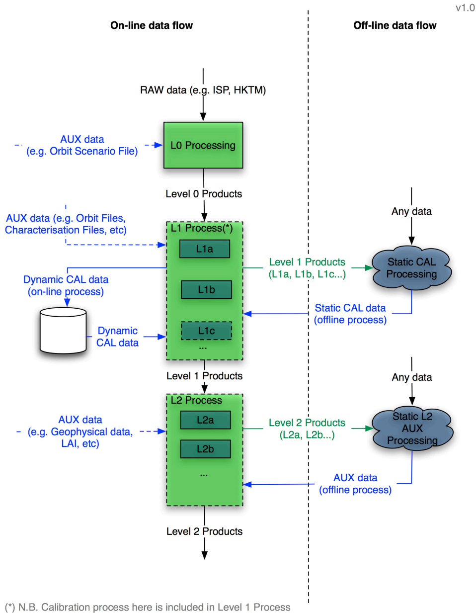
Fig. 3-6 Generic view of dataflow in an Earth Observation data processing Ground Segment
