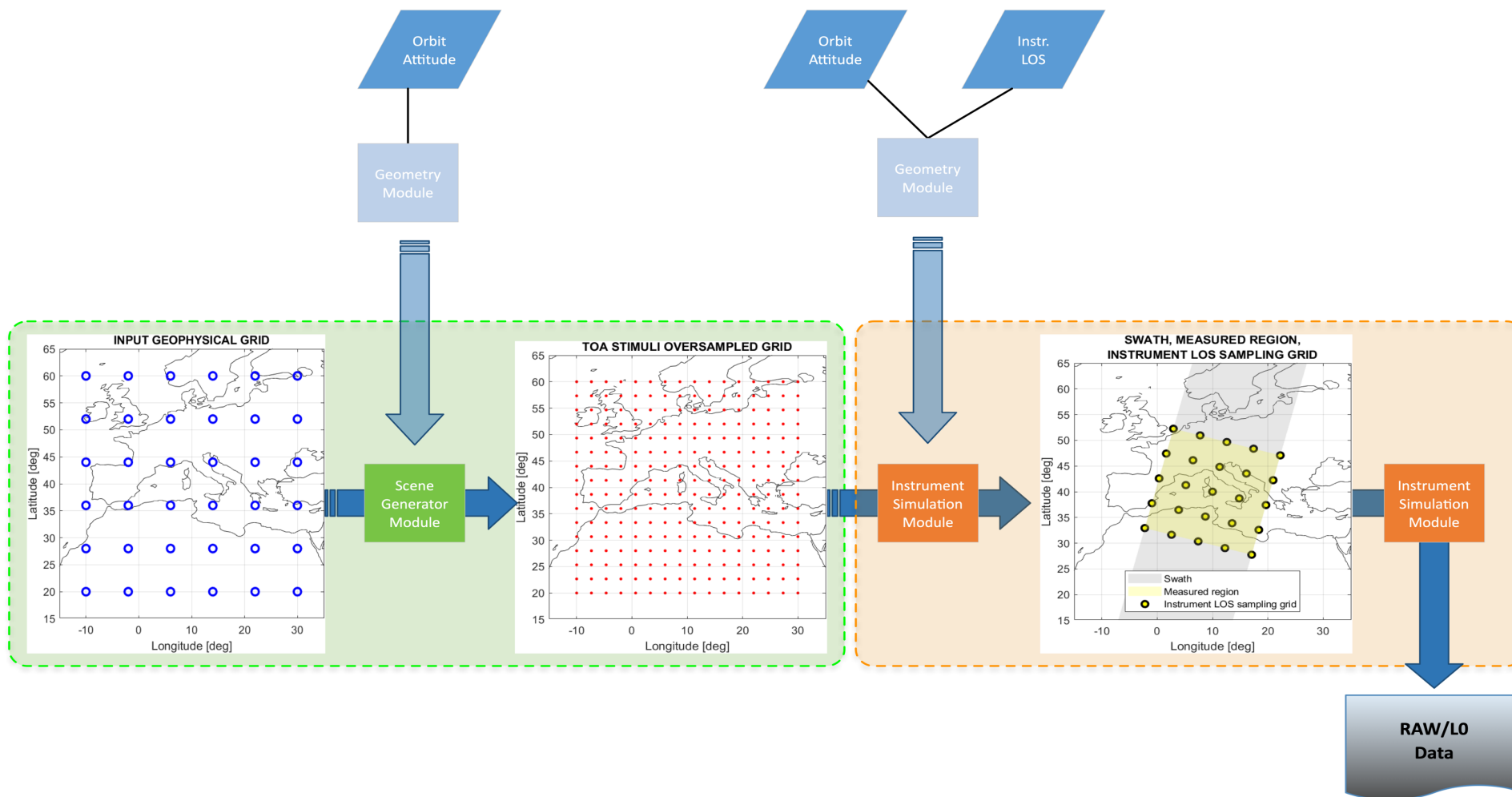
Fig. 3-3 reference architecture of SGM interfaces.
