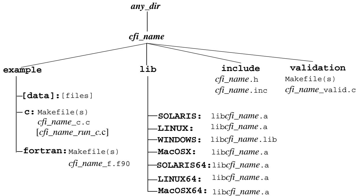
Figure 6: CFI directories structure
