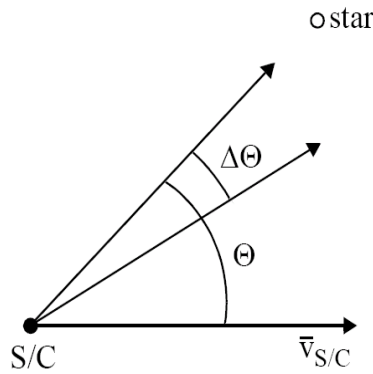
Figure 16: Satellite aberration
