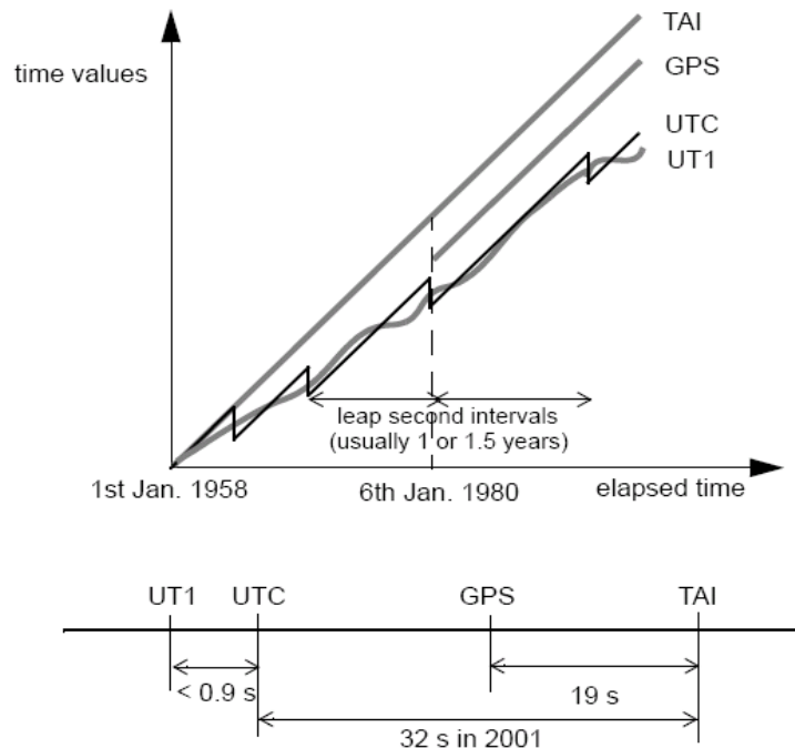
Figure 1: Relationships between UT1, UTC and TAI
