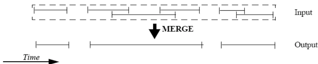
Figure 13: xv_timesegments_compute_merge function
